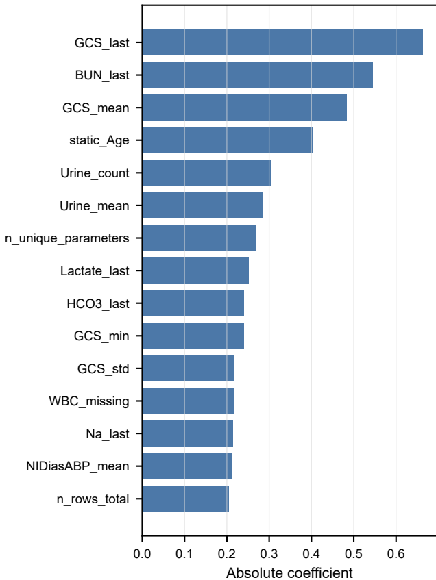
Logistic Regression coefficients
